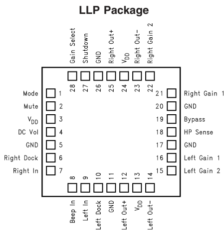
Top View Order Number LM4835LQ See NS Package LQA028AA for Exposed-DAP LLP
