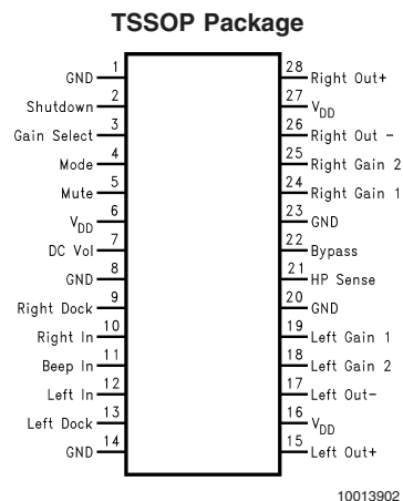
Top View Order Number LM4835MT or LM4835MTE See NS Package MTC28 for TSSOP or See NS Package MXA28A for Exposed-DAP TSSOP
